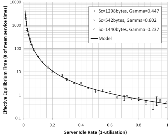
Figure 1. Simulated equilibrium time lag measured for three traffic profiles compared with the model. (Data points represent the average of 5 runs of 1,000 independent simulations. Error bars indicate 95% confidence intervals.)
