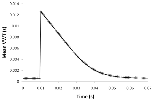
Figure 2. Mean VWT profiles. The link bandwidth in all four experiments was 1Mbit/s. (Data points represent the average of 2000 simulations, solid lines represent model predictions.)
