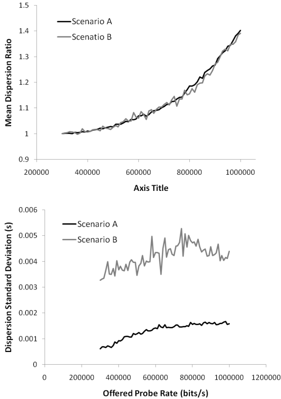
Figure 5. Probing results obtained from two network scenarios: (A) A two-hop path carrying 50byte packets and (B) a one-hop network path carrying 800byte packets. The mean dispersion ratios are practically identical, but the standard deviations significantly different. (Offered probe rate=probe packet size/packet separation)
